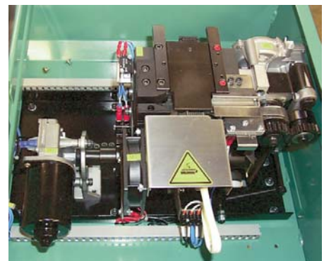
Compact mechanical control head
